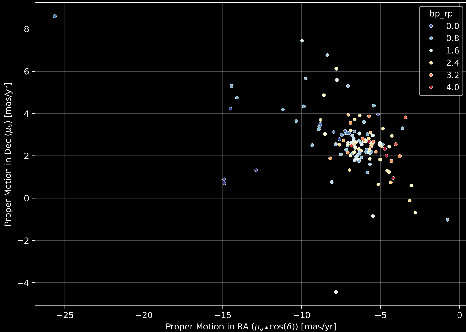
APOGEE DR17 Field: [287-01-C] Proper Motion Diagram (n= 138)
