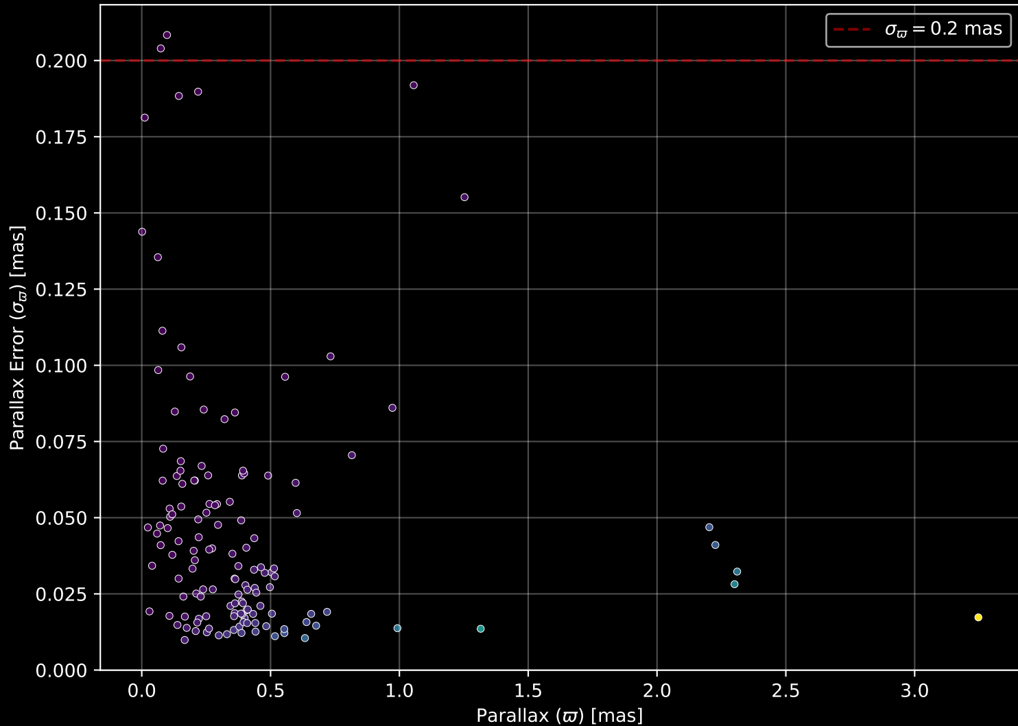
APOGEE DR17 Field: [287-01-C] Parallax Quality (n= 138)
