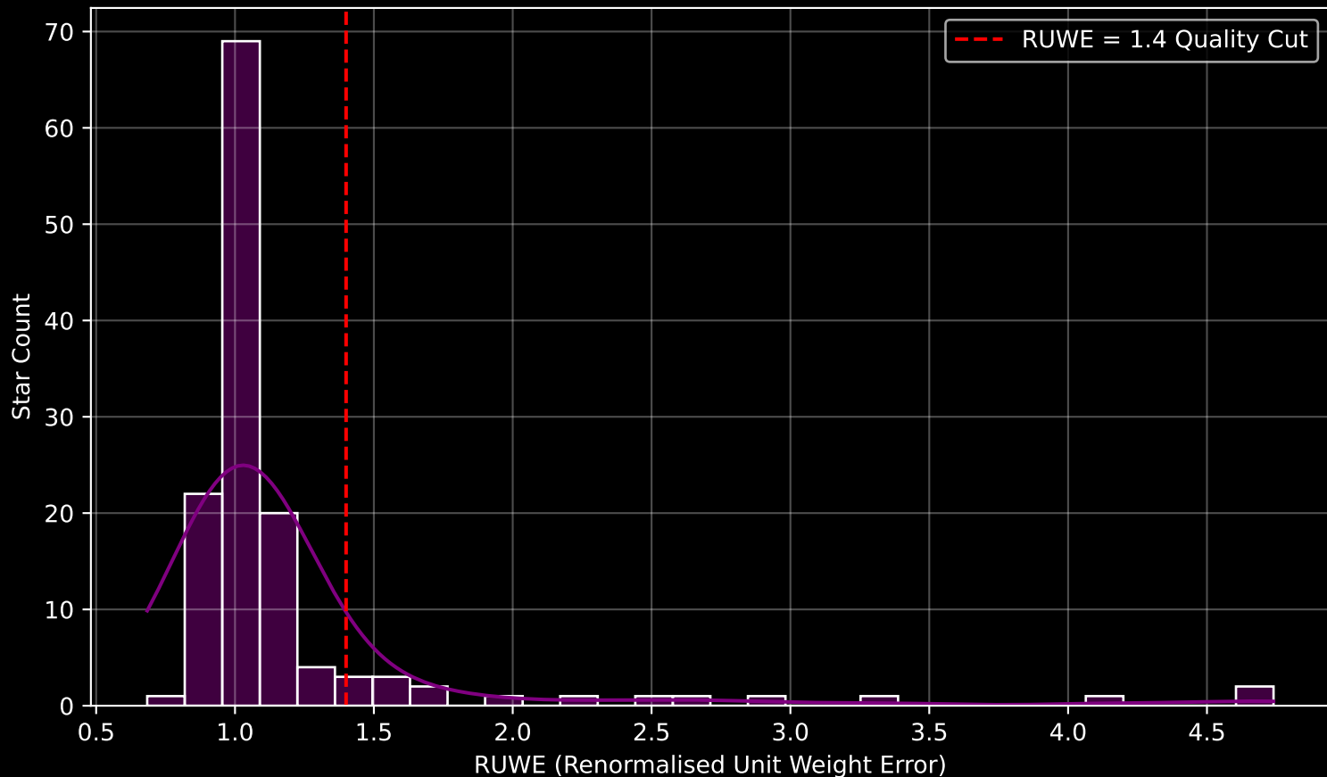
GAPOGEE DR17 Field [287-01-C] RUWE Distribution (n= 133)
