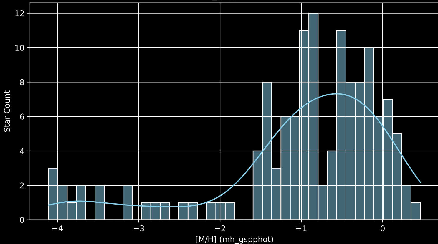
APOGEE DR17 Field: [287-01-C [M/H] (mh_gspphot) (n= 134)
