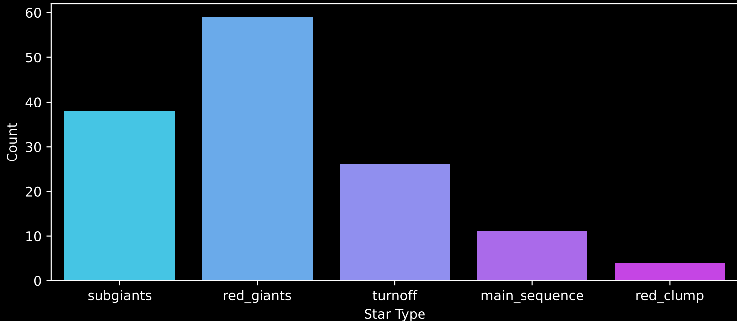
APOGEE DR17 Field: [287-01-C] Count plot of Star Type
